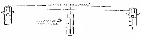
Fig. 5432. STANDARD DATA FOR IRON BRAKE-BEAM.
